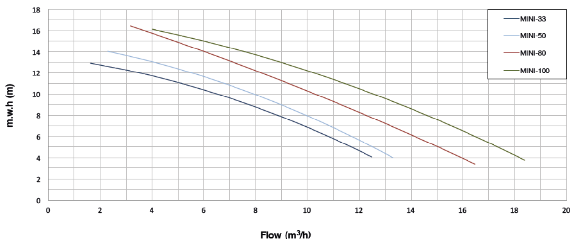
Characteristics curve
