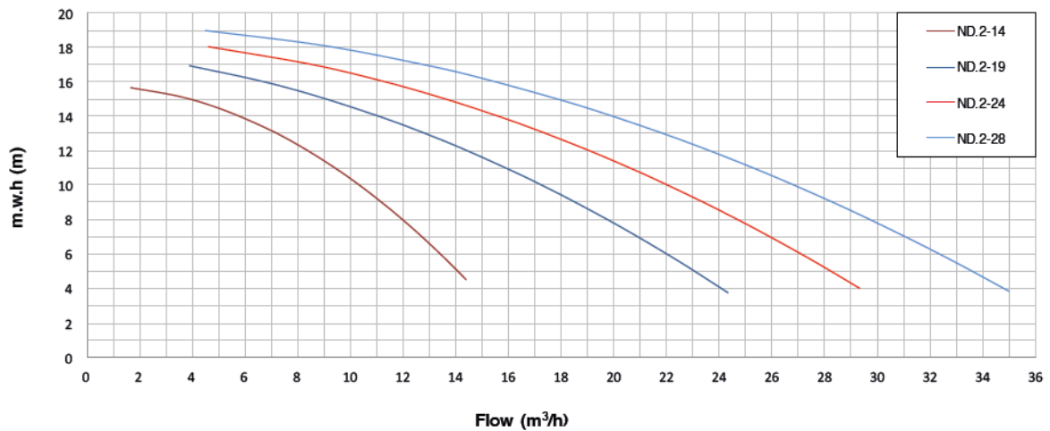
Characteristics curve
